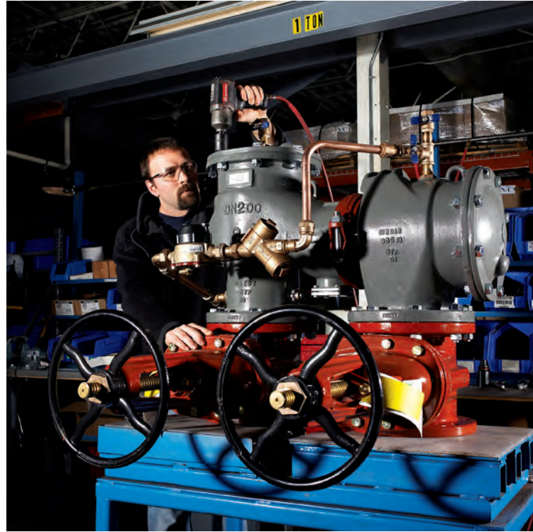
FEBCO large-diameter backflow preventer final assembly in Franklin, New Hampshire.
