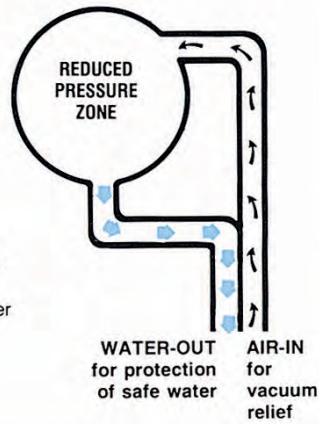
Fig. 2 Schematic of Watts Series 909 "How it works".
