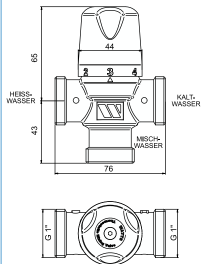
MMV-C 25
