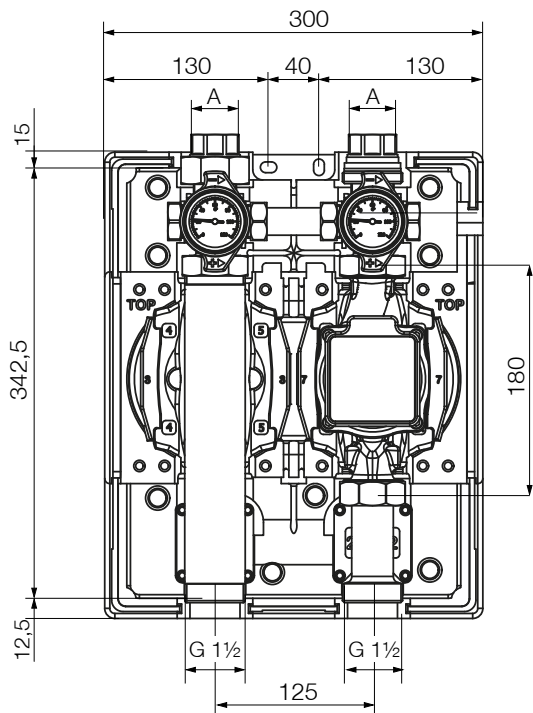
FlowBox HK25/32
