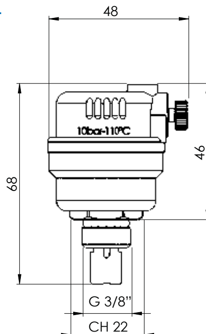
MHL
