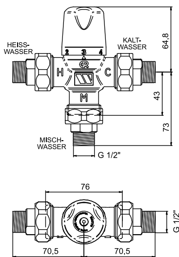
MMV-C 15
