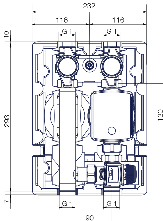
FlowBox HKF20
