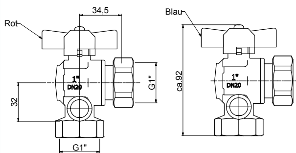
KHT-SET ECK
