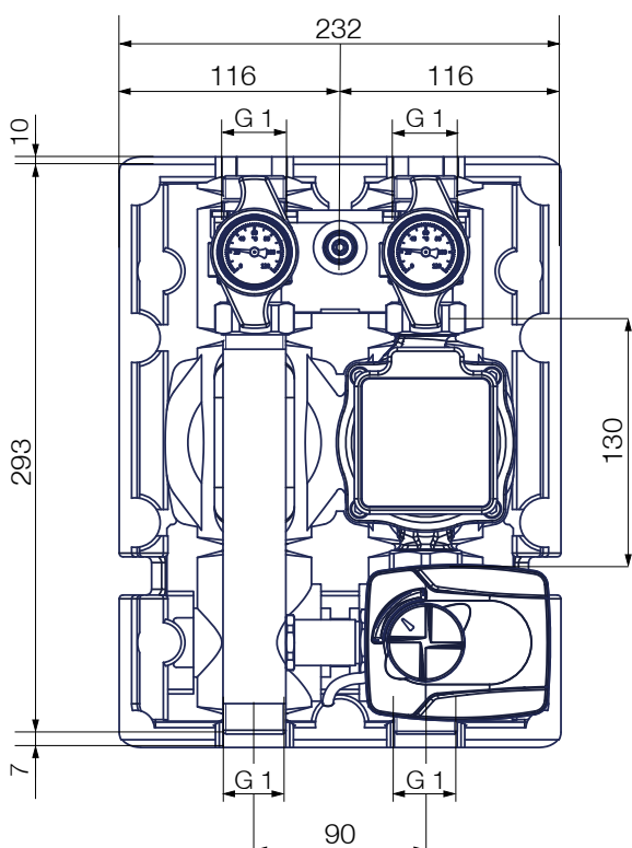
FlowBox HKM20
