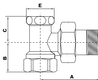
RLE
