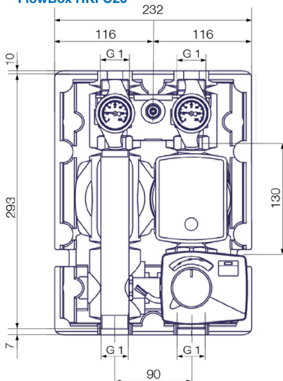
FlowBox HKFC20
