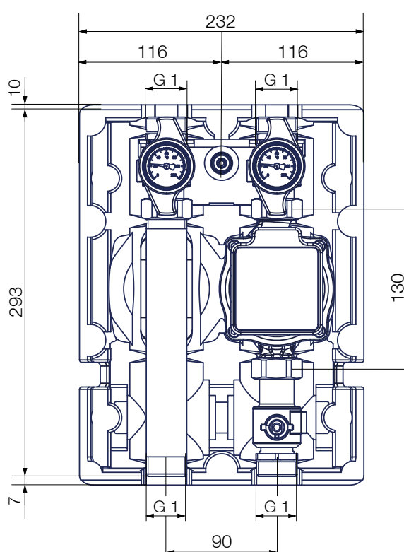
FlowBox HK20-KH
