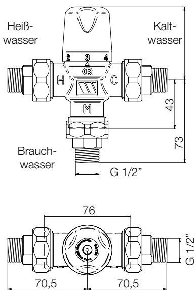
MMV-S 15
