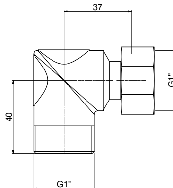
Winkel Set
