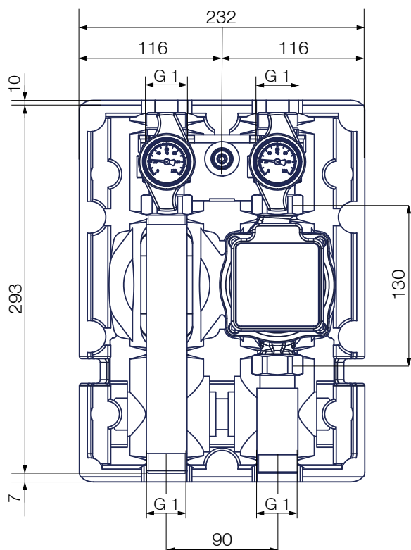
FlowBox HK20
