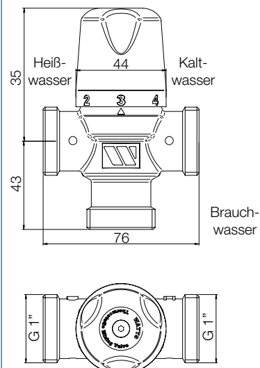
MMV-S 25
